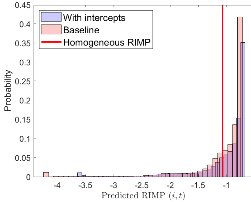
Figure A.7: Robustness to group-specific intercepts – predicted distribution
