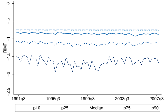
Figure A.1: Moments of the predicted RIMP distribution over time
