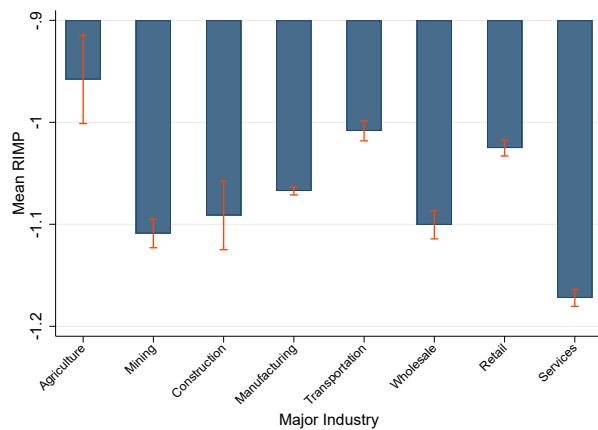
Figure A.4: RIMP heterogeneity by industry
