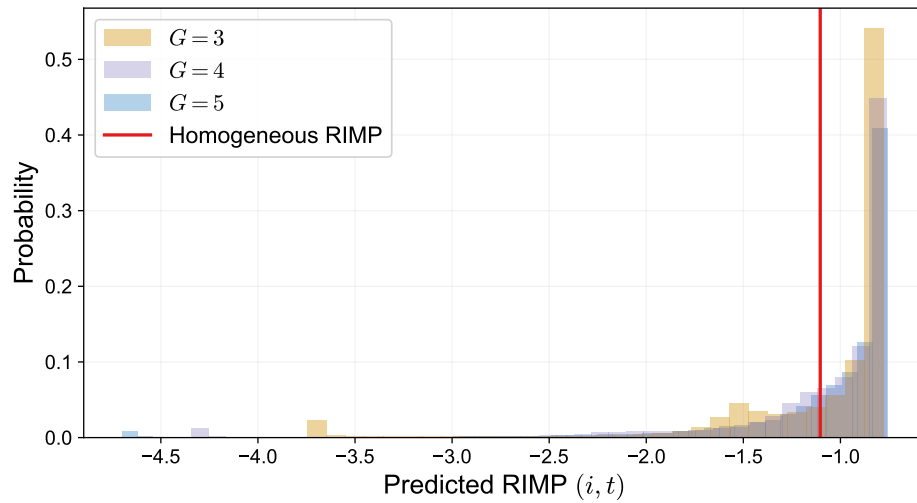
Figure A.6: Predicted RIMP distributions for different G
