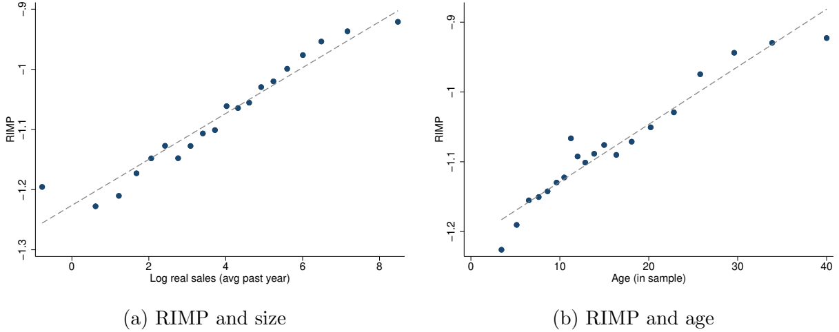
Figure 3: RIMP heterogeneity by firm size and age
