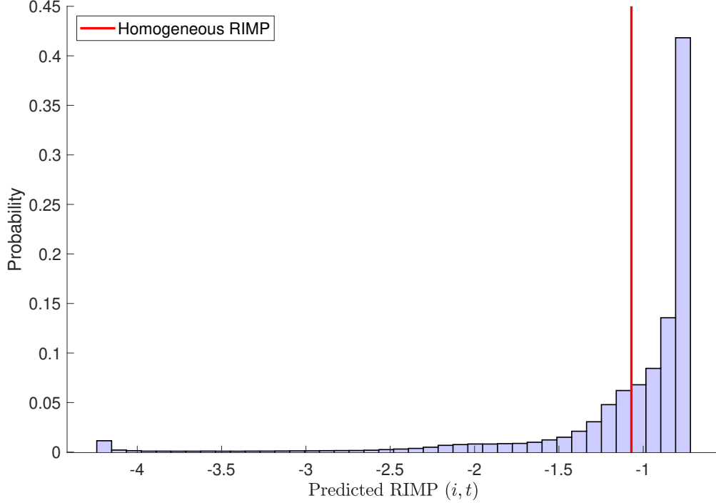
Figure 1: Investment responses to monetary policy tightening – predicted distribution
