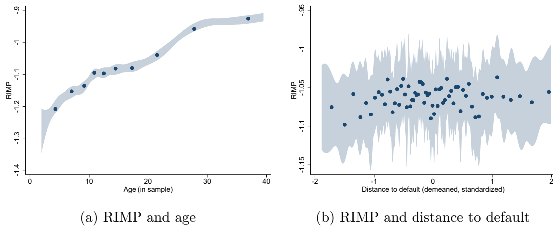
Figure A.3: RIMP heterogeneity by firm age and distance to default
