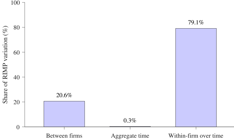
Figure 2: Sources of variation in investment responses to monetary policy
