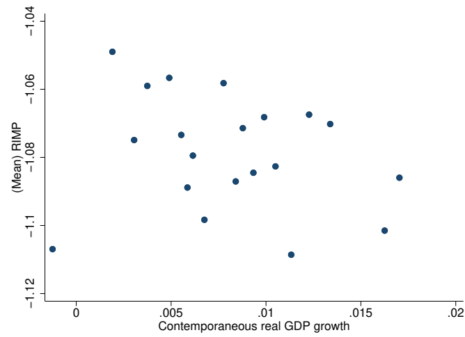
Figure A.2: Average RIMP and real US GDP growth
